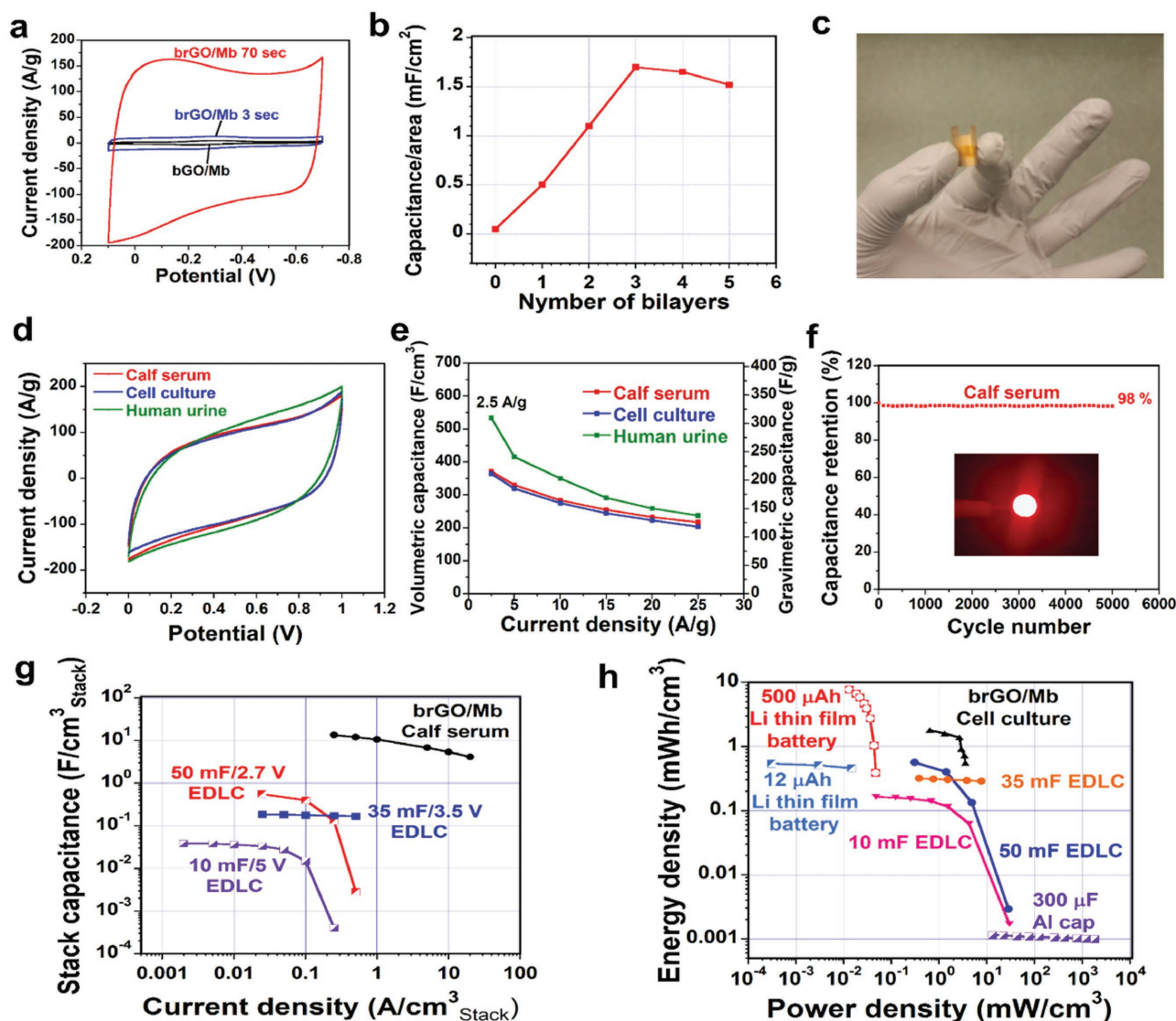
Figure 4. Electrochemical behavior of a brGO/Mb BEC. a) Cyclic voltammetry (CV) at 300 \text{ mV s}^{-1} of nonreduced film (bGO/Mb), and electrochemically reduced film (brGO/Mb) for 3 and 70 s. b) Optimization of the film capacitance with the number of bilayers showing the highest capacitance for three bilayers. c) Photograph of the packageless brGO/Mb EC. d) Cyclic voltammetry at 1000 \text{ mV s}^{-1} of brGO/Mb film in different electrolytes. e) Change of volumetric and gravimetric capacitance with moderate-to-high current density for a brGO/Mb electrode in biofluids. f) Cyclic stability of the brGO/Mb BEC in calf serum, inset shows LED powered by three brGO/Mb BECs connected in series with calf serum saturated separators. g) Volumetric stack capacitance of a brGO/Mb BEC at different current densities as compared to commercial electrical double layer capacitors (EDLC). h) Energy and power densities of a brGO/Mb BEC in a cell culture medium as compared to commercial EDLC, 300 \mu\text{F}/3 \text{ V} aluminum electrolytic capacitor, 12 \mu\text{Ah}/3.3 \text{ V} Li thin film battery, and 500 \mu\text{Ah}/5 \text{ V} Li thin film battery.
