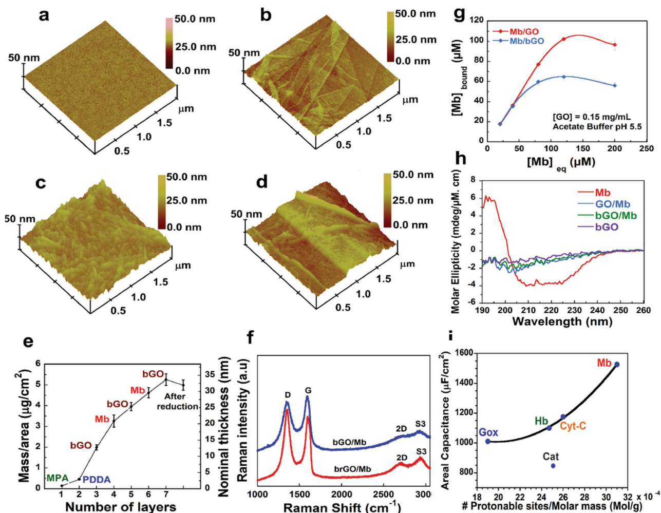
Figure 3. Characterization of the graphene–protein hybrid electrodes. a–d) Tapping mode AFM images of the layer-by-layer assembled film on a mica disc. a) PDDA, b) PDDA-bGO, c) PDDA-bGO-Mb, and d) PDDA-bGO-Mb-bGO. e) Change in the mass/area and nominal thickness of the film as a function of the number of layers assembled as measured by quartz crystal microbalance (QCM). f) Raman spectra of films before and after electrochemical reduction. g) Myoglobin binding to GO (red curve) and bGO (blue curve) in 10 \times 10^{-3} M acetate buffer at pH 5.5 as a function of increasing concentrations of myoglobin. h) Circular dichroism spectra suggesting extensive denaturation of Mb upon binding to either GO or bGO. i) Areal capacitance of three bilayers of brGO/protein in correlation to the number of sites available for protonation/deprotonation normalized by the molar mass of proteins. Cyt-C, Mb, Hb, GOx, and Cat stand for cytochrome-C, myoglobin, hemoglobin, glucose oxidase, and catalase, respectively. The highest areal capacitance among these proteins was observed with brGO/Mb film.
